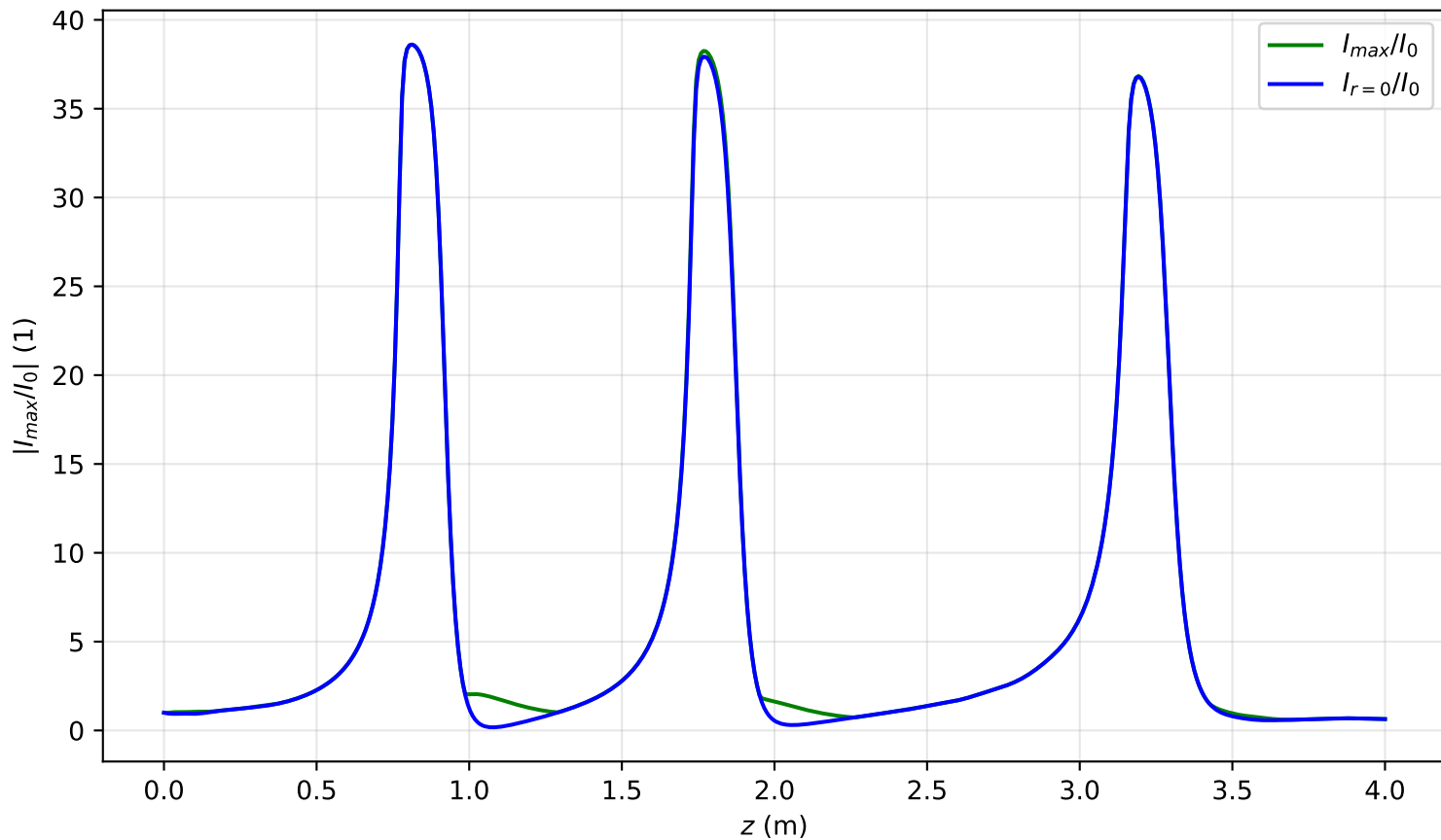
I_{max}(x = 0, y = 0, z)/I_0 , Pin=2.8Pcr, noisy input, artificial time
